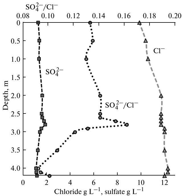
Fig. 8. Chloride and sulfate ion concentrations, their ratio in the water and pore water of sediments in Lake Kисло-Sladkoe.
